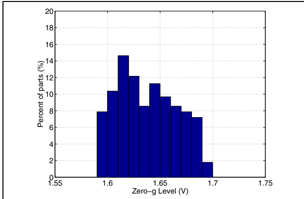
Figure 7. z-axis Zero-g level at 3.3V
