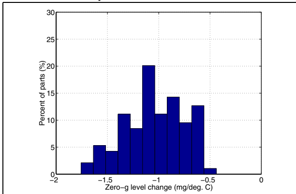
Figure 13. z-axis Zero-g level change Vs temperature
