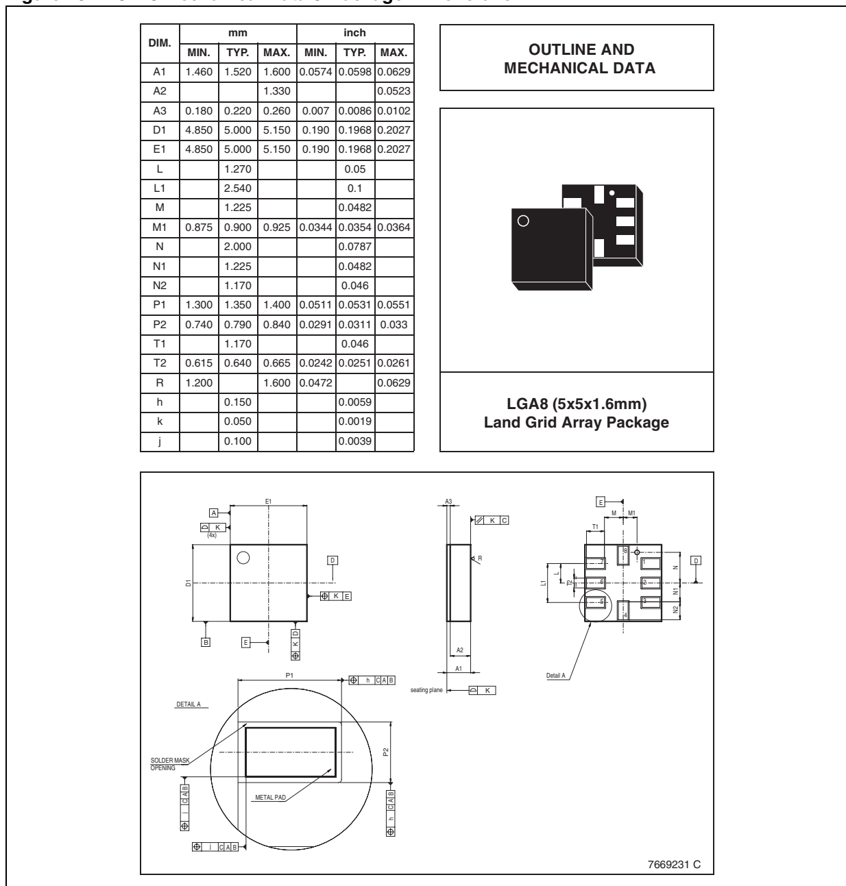
Figure 20. LGA-8 Mechanical Data & Package Dimensions
