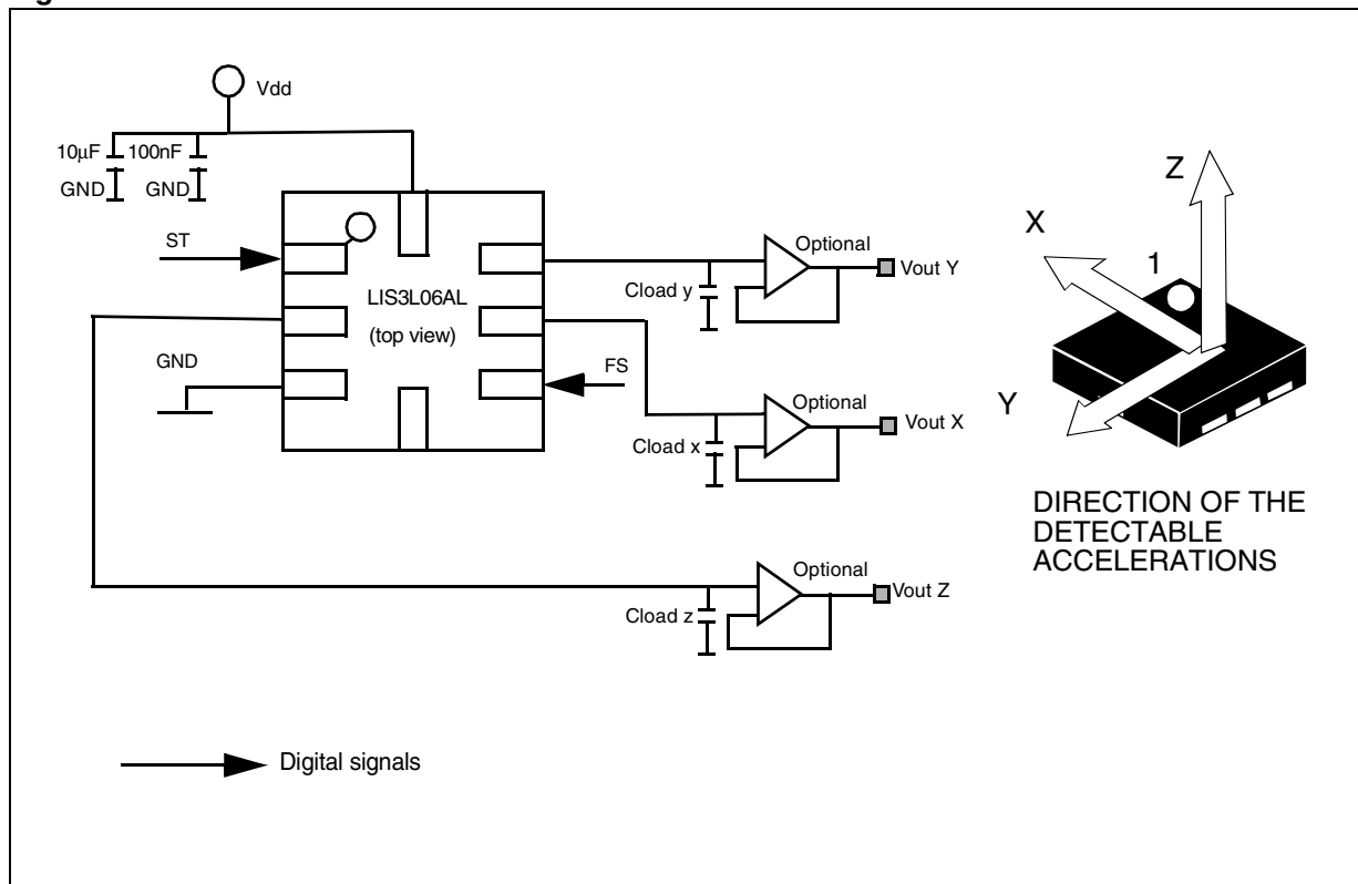
Figure 3. LIS3L06AL Electrical Connection
