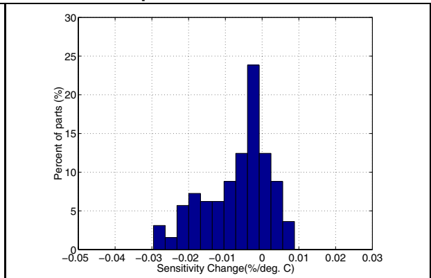
Figure 14. x-axis sensitivity change Vs temperature
