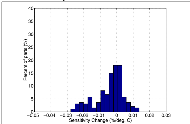
Figure 15. y-axis sensitivity change Vs temperature
