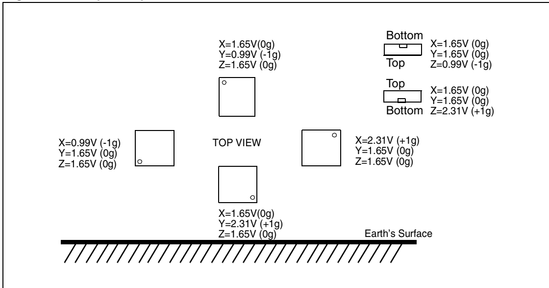
Figure 4. Output response vs Orientation
