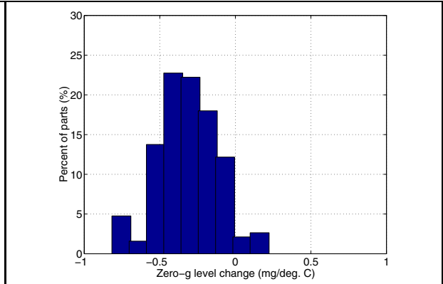
Figure 12. y-axis Zero-g level change Vs temperature
