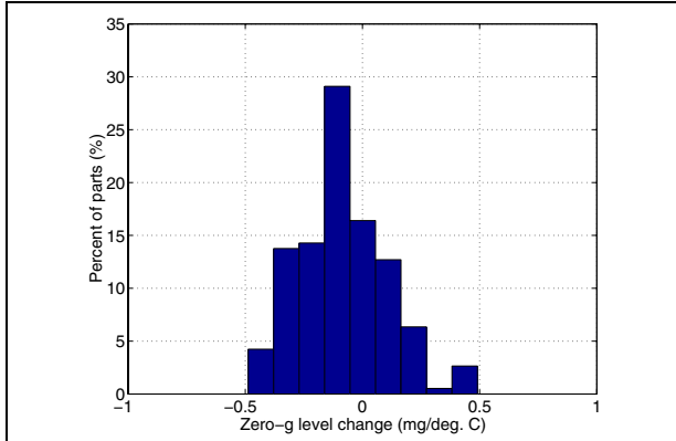
Figure 11. x-axis Zero-g level change Vs temperature
